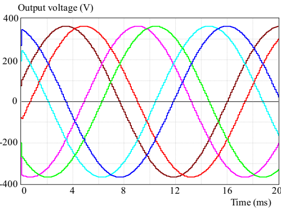
Fig. 6. Six-pulse autotransformer output voltage
