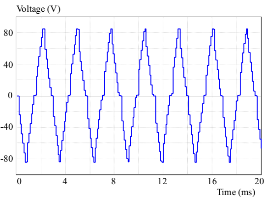
Fig. 7. Voltage waveform across the double-tap IPR
