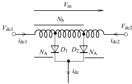
Fig. 5. Tapped inter-phase transformer circuit
