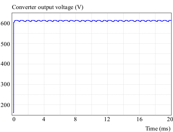
Fig. 9. 24-pulse ac-dc converter output voltage
