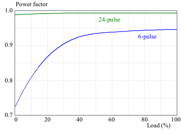
Fig. 12. Variation of power factor with load on DTCIMD in 6-pulse, 12-pulse and 24-pulse ac-dc converter
